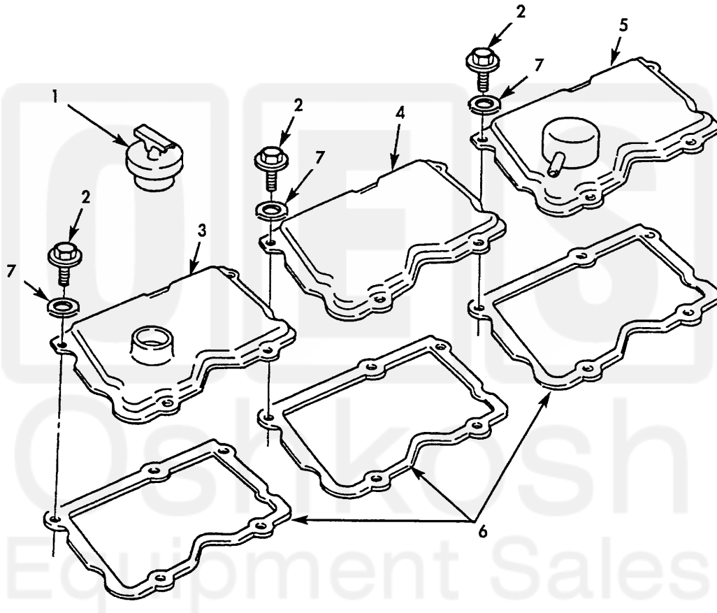
Figure 9. Rocker Cover.
